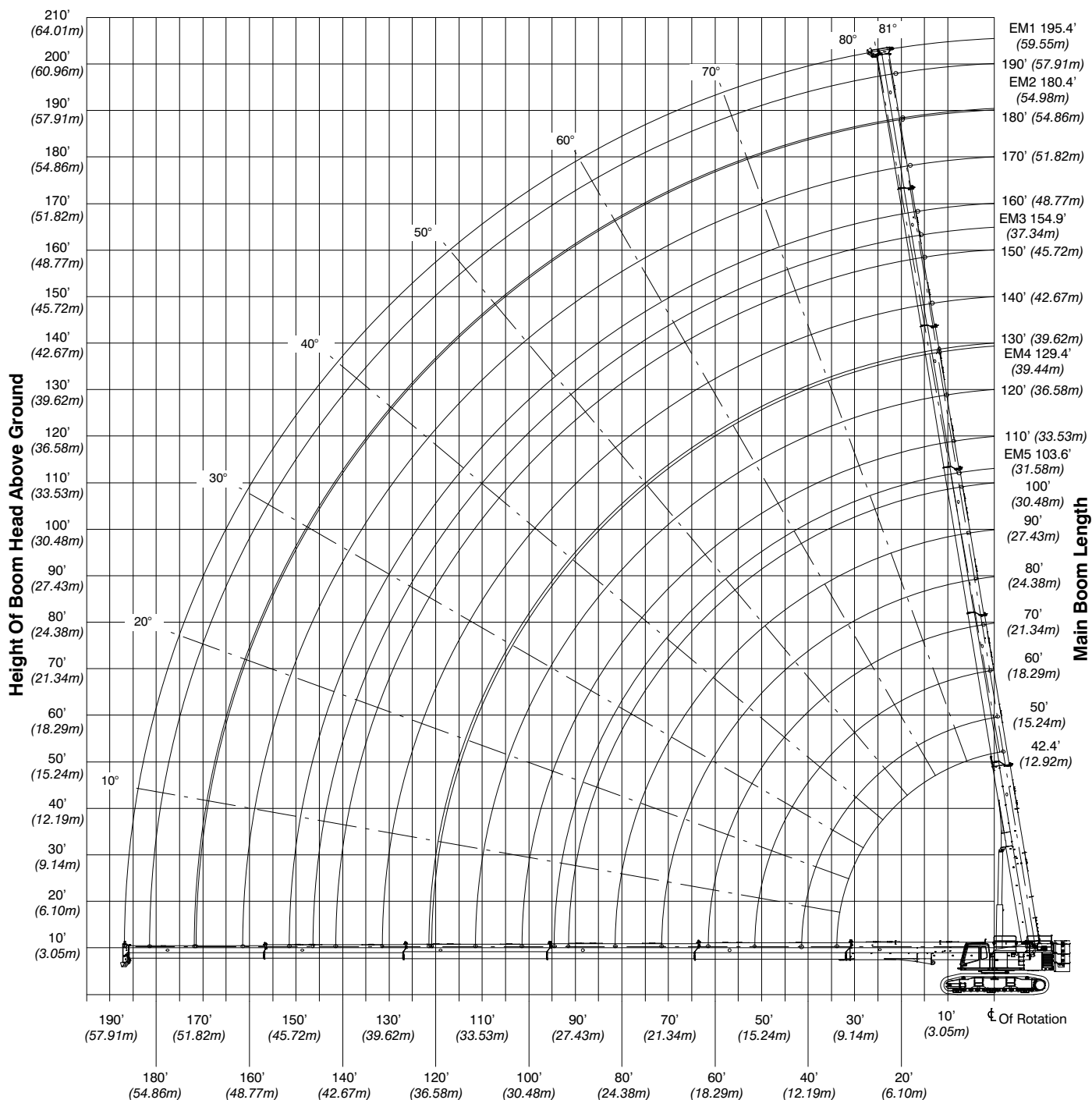
Operating Radius From Centerline Of Rotation
