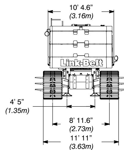
Retracted Gauge
