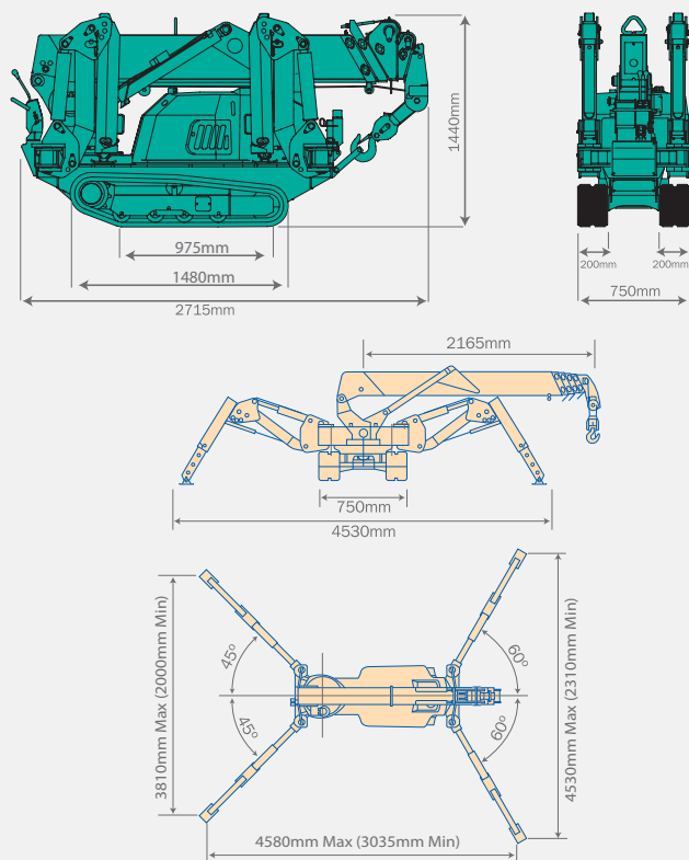
Diagram shows outriggers at maximum position
