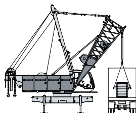
Unloading and assembly of crawler side frames
