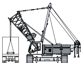
Unloading and assembly of carbody counterweight
