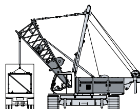
Unloading and assembly of boom
