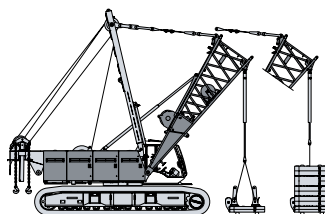
Unloading and assembly of rear counterweight
