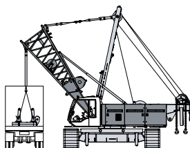
Unloading and assembly of rear counterweight
