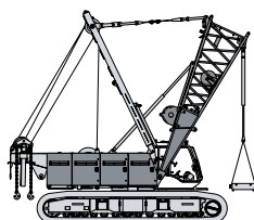
Unloading and assembly of carbody counterweight
