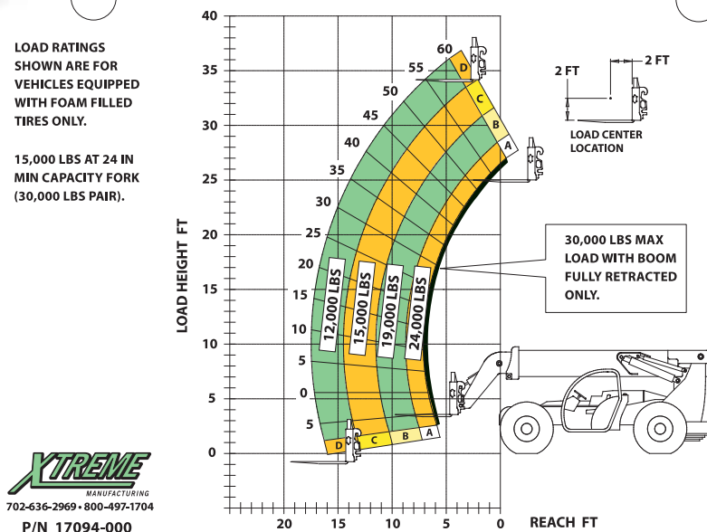
XR3034 LOAD CHART - STANDARD 6FT CARRIAGE
