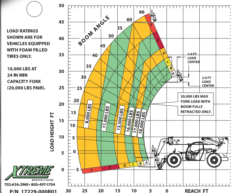
XR2045 LOAD CHART OUTRIGGERS DOWN - STANDARD CARRIAGE
