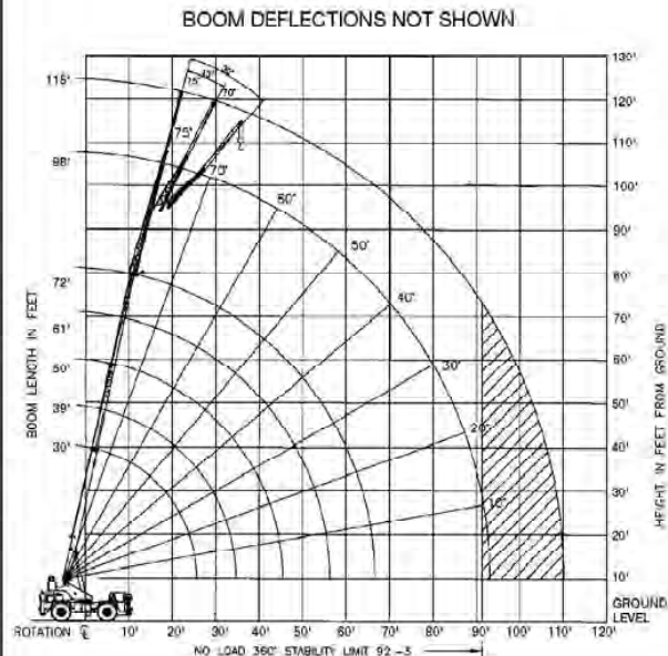
Range Diagram (30'-72' boom)
