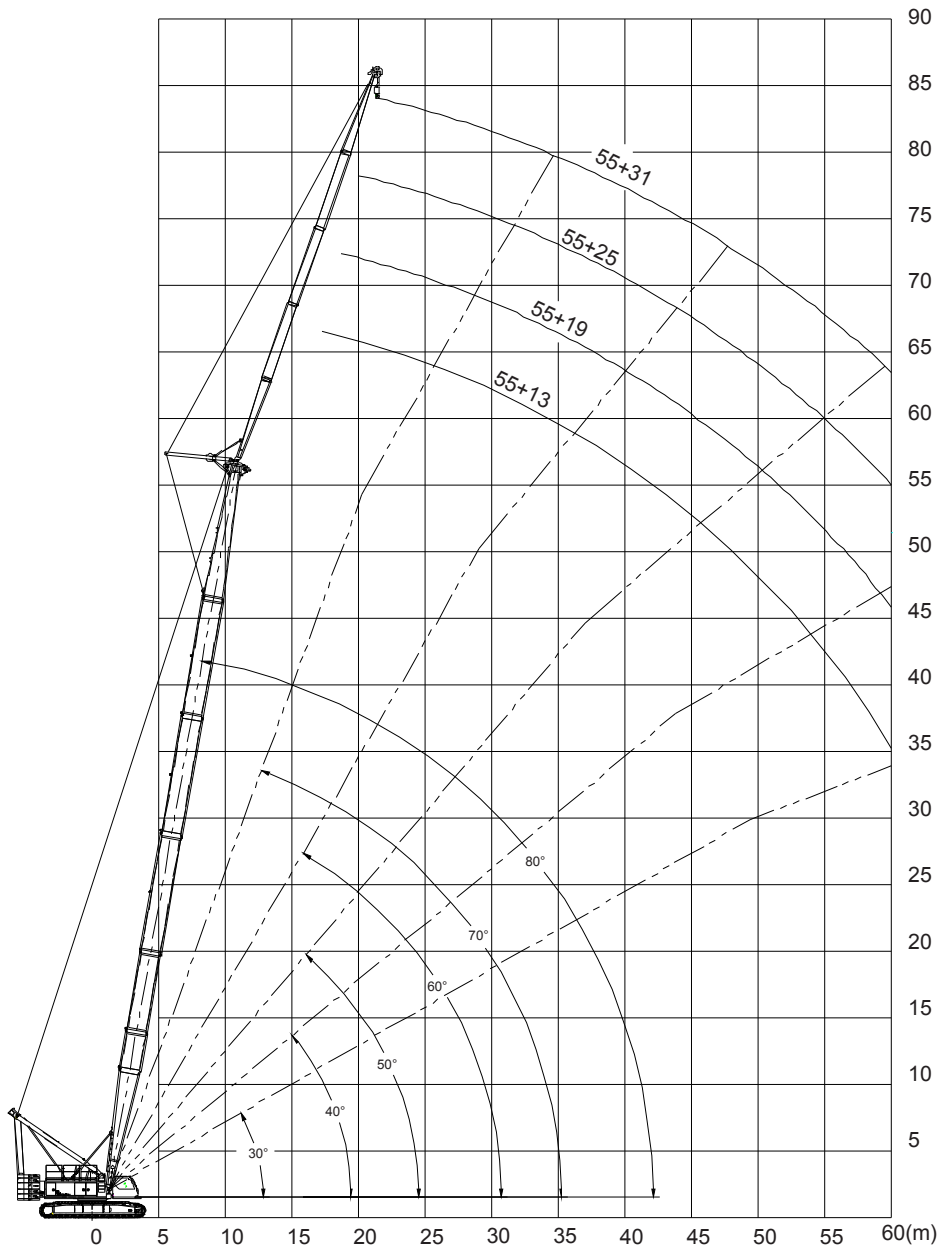
Main Boom + Fixed Jib Lifting Height Characteristics Curve (I)
