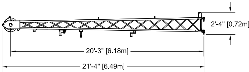
21.0ft (6.4m) JIB POINT WEIGHT: 1351 lb (613 kg)
