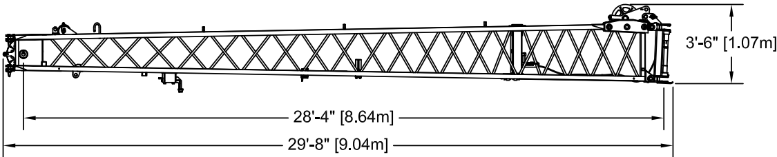
28.9ft (8.8m) BASE JIB WEIGHT: 1351 lb (613 kg)
