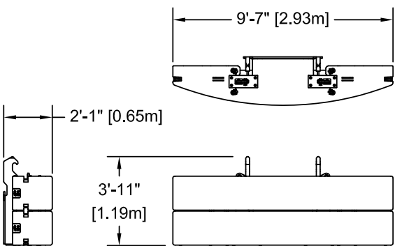
STANDARD COUNTERWEIGHT WEIGHT: 17,400 lb (7893 kg)
