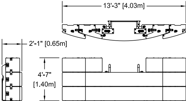
HEAVY COUNTERWEIGHT (OPTIONAL) WEIGHT: 28,200 lb (12,791 kg)
