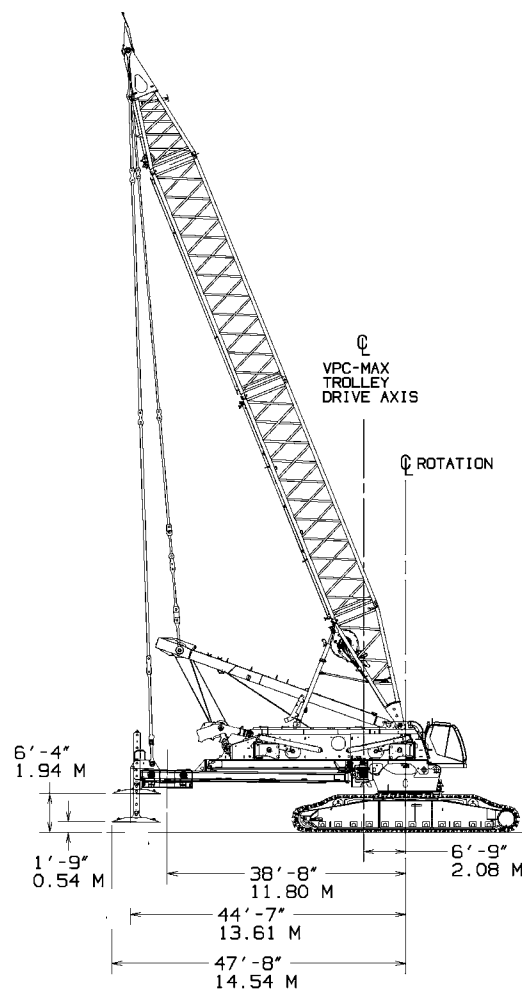
VPC-MAX BEAM: MIN POSITION CWT TRAY: MAX POSITION
