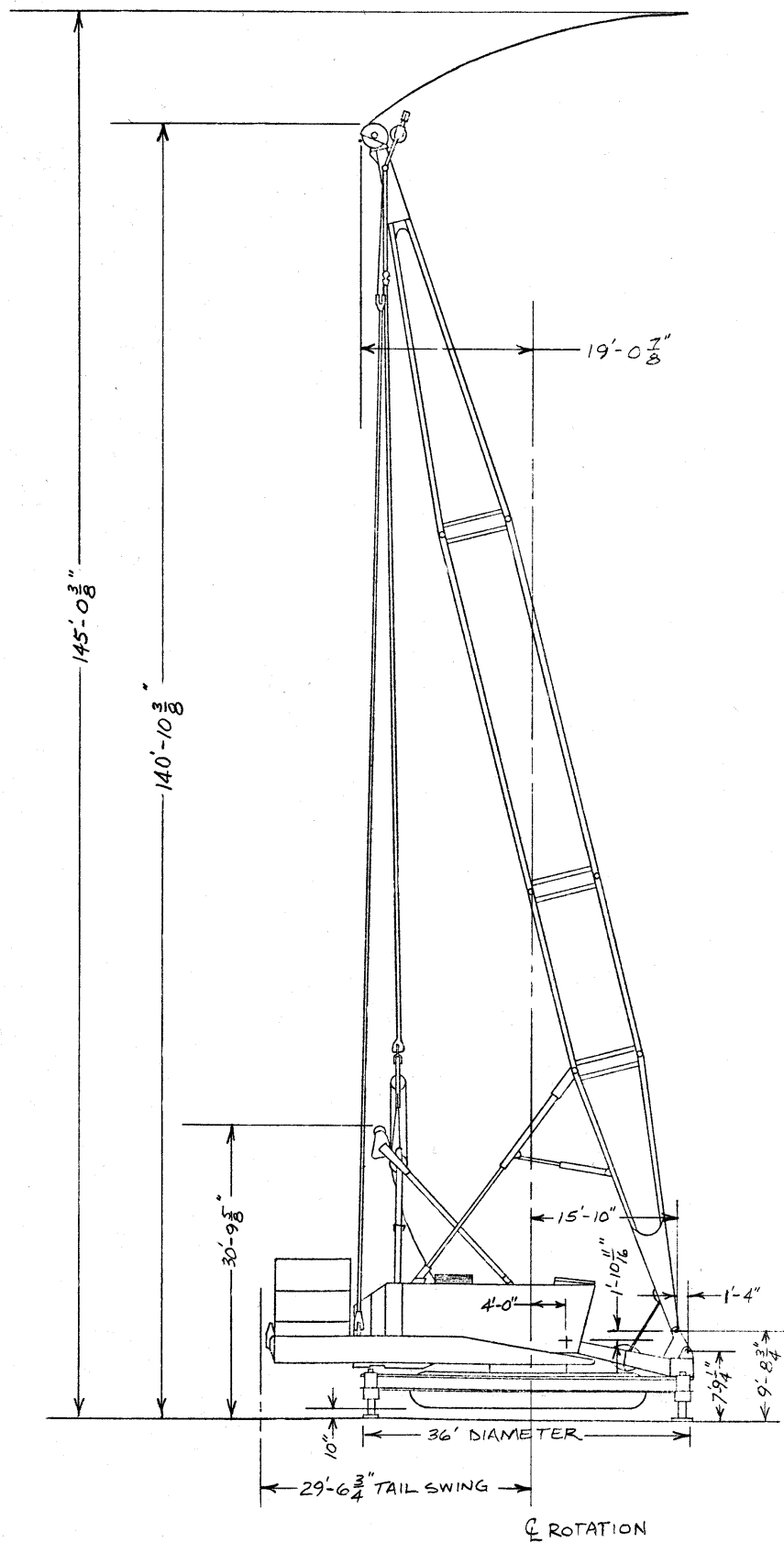
OUTLINE DIMENSIONS 4100W RINGER
