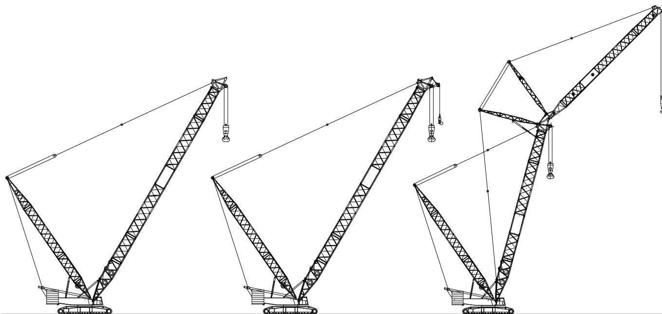
SL-N Heavy Duty 118.1-315 ft (36.0-96.0m)
