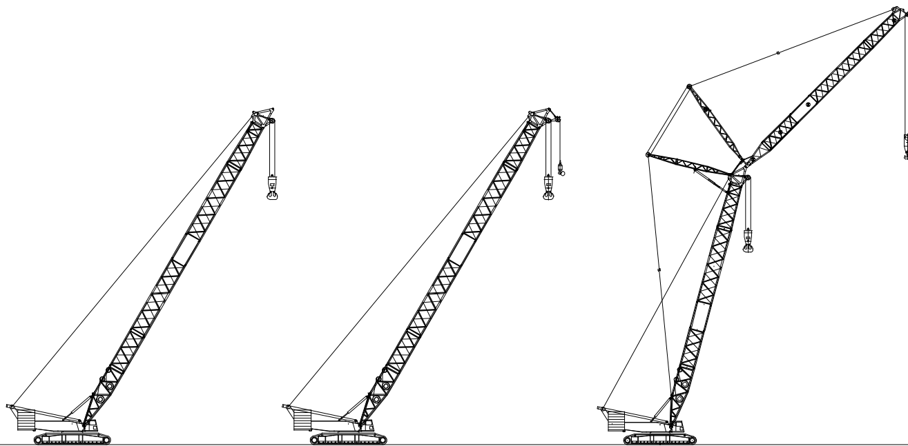
78.7–315.0 ft (24.0–96.0m) Standard Heavy Duty Boom
