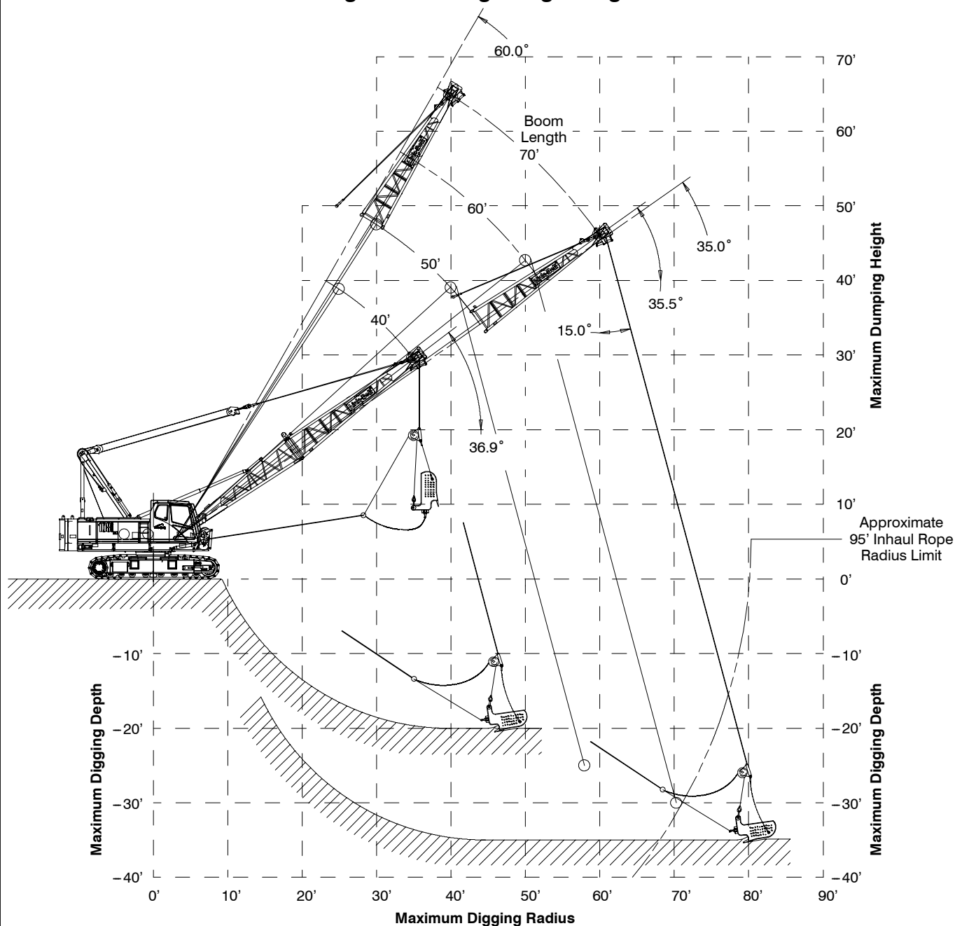
Dragline Working Range Diagram
