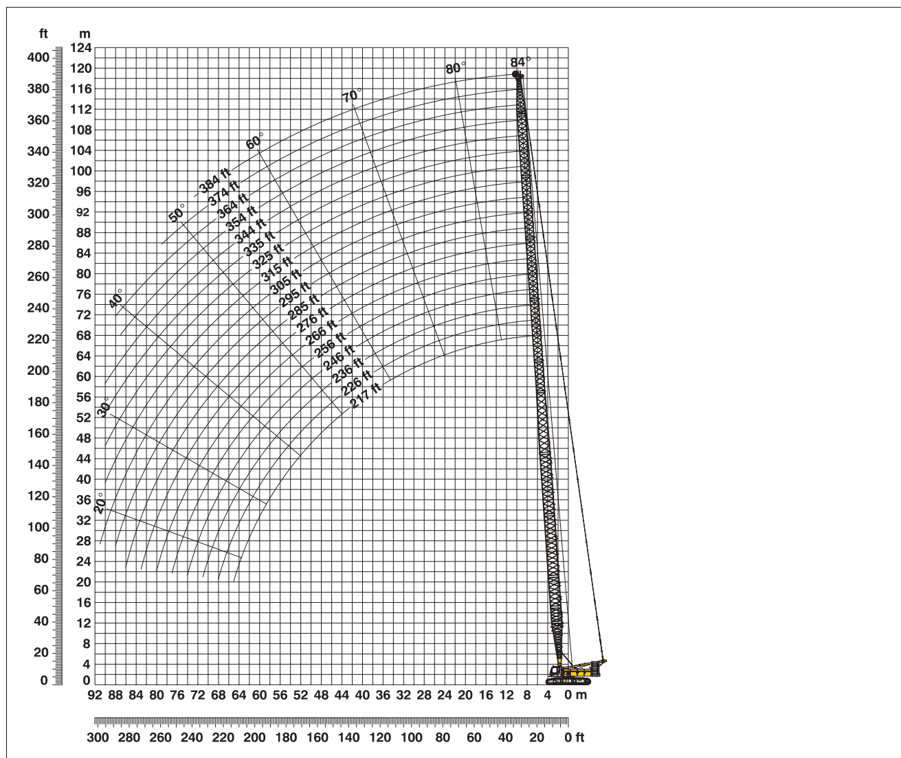
Configuration for L – boom lengths (217 ft – 384 ft)
