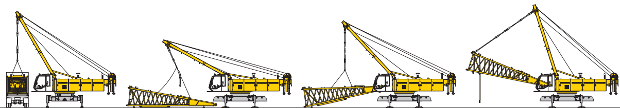
Unloading and assembly of boom foot
