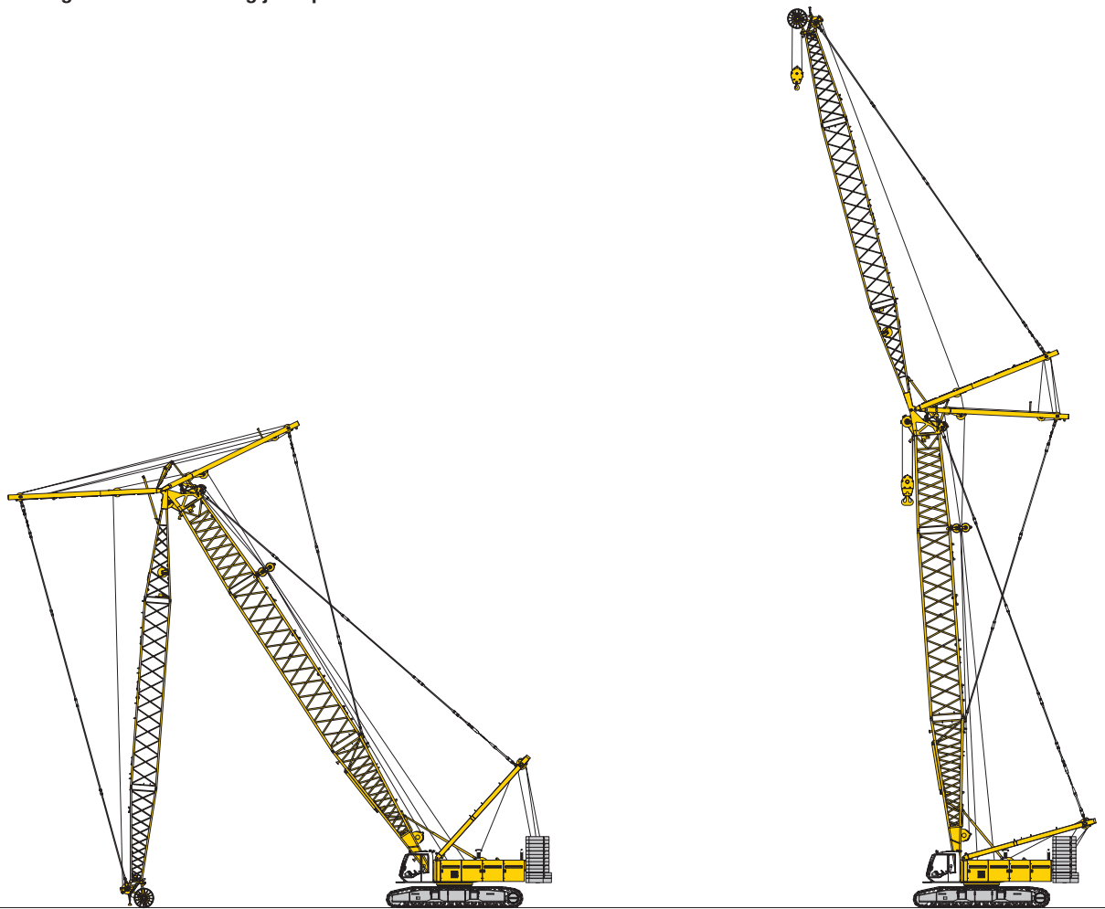
Erecting of main boom and luffing jib
