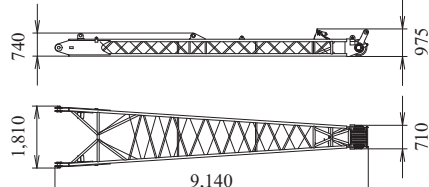
Rear Strut (Luffing Jib) Weight: 1,510 kg
