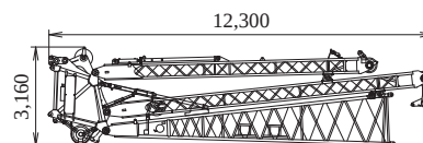
Luffing Boom Tip Assembly Weight: 6,730 kg
