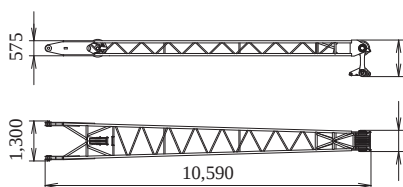
Front Strut (Luffing Jib) Weight: 1,410 kg
