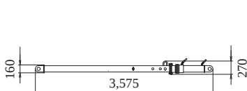
Strut Backstop (Luffing Jib) Weight: 180 kg
