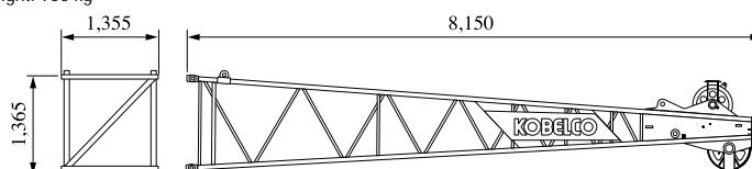
Tower Jib Top
