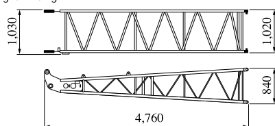
Jib Base (For Crane)
