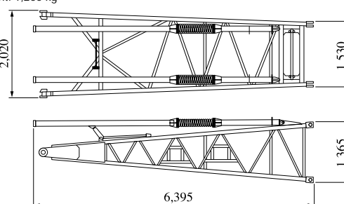
Tower Jib Base
