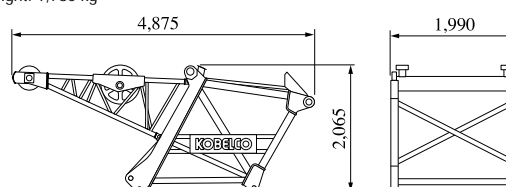
Tower Cap
