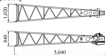
Jib Base (For Crane)
