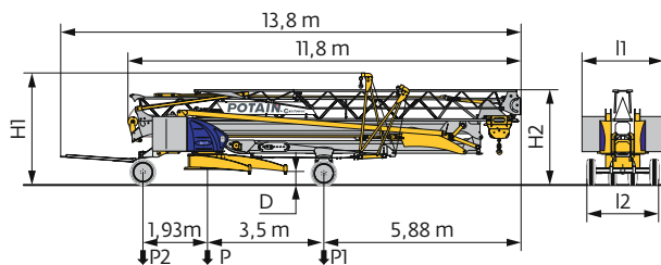
DS62/S81 - DS65/S65
