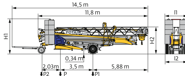
DJ126M/S125
