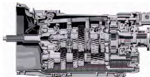
Daimler Chrysler 16 speed G240-16
