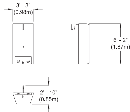
Counterweight Segment "C" 2 Pieces Weight: 11,670 lb (5,300kg) each
