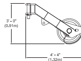
Auxiliary Nose Sheave Weight: 298 lb (135 kg)
