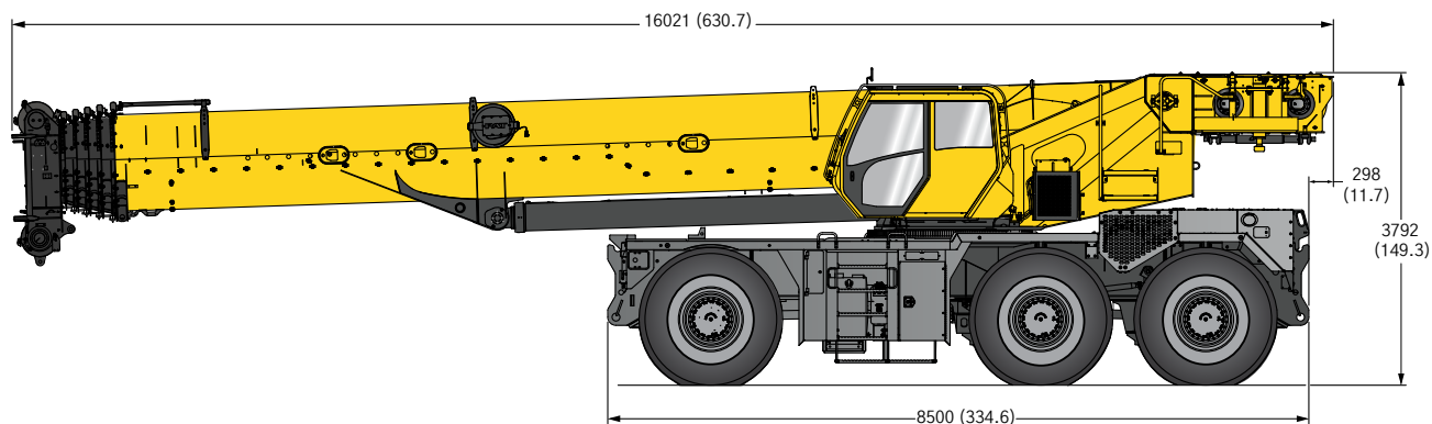
TRANSPORT DIMENSIONS OUTRIGGER BOXES AND COUNTERWEIGHT REMOVED
