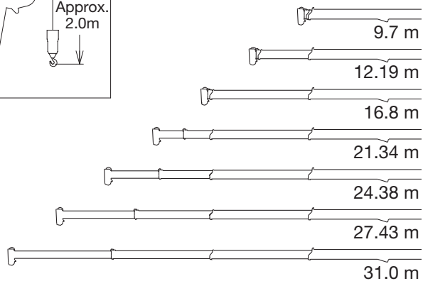
Boom Length
