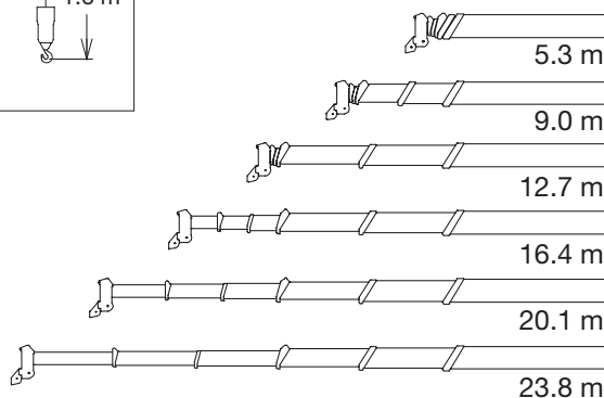
Boom Length
