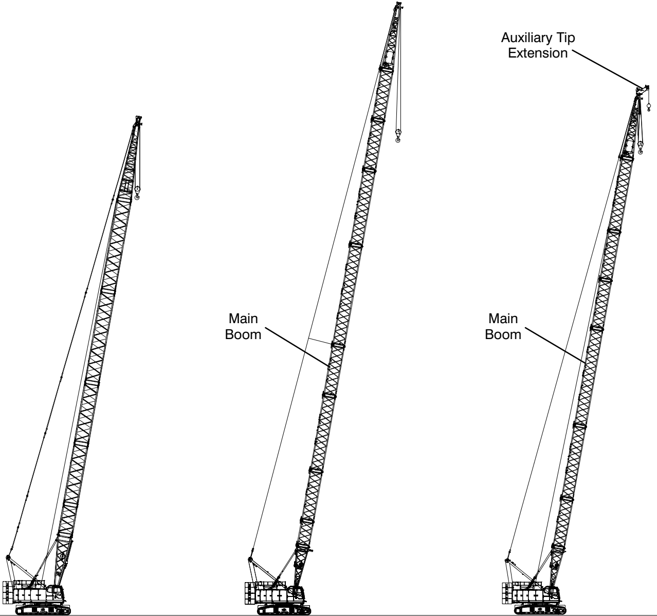
45–155 ft (13.72–47.74m) Main Angle Boom
